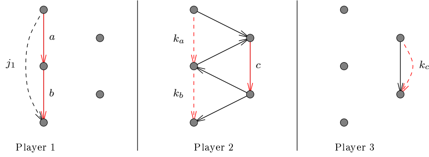
Figure 1: A path whose realization cannot be represented by an arborescence. Black denotes normal and red denotes contractual; a solid line is an arc while a dotted line is a demand. In the unique realization of the path ab , the sink, which corresponds to the single-arc path in the network of player 3, has in-degree 2.
